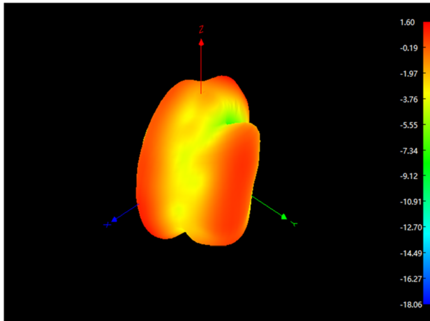
Radiation Pattern at 2500MHz of Antenna
