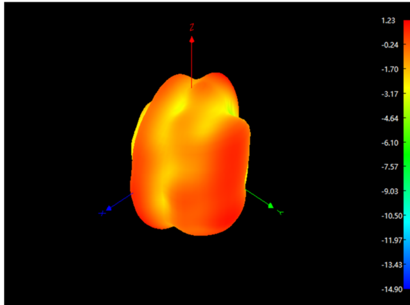
Radiation Pattern at 2400 MHz of Antenna
